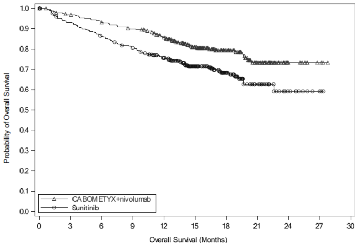
Figure 6: Kaplan-Meier Curve of Overall Survival in CHECKMATE-9ER
