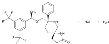
rolapitant hydrochloride
