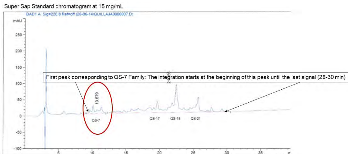
Figure C2-1 Super Sap Standard Chromatogram
