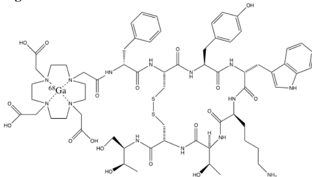
Figure 1: Chemical Structure of Ga 68 DOTATOC
