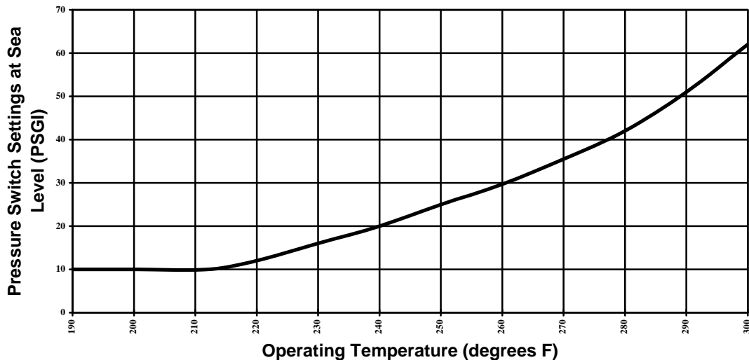
Figure 57. Pressure Switch Setting
