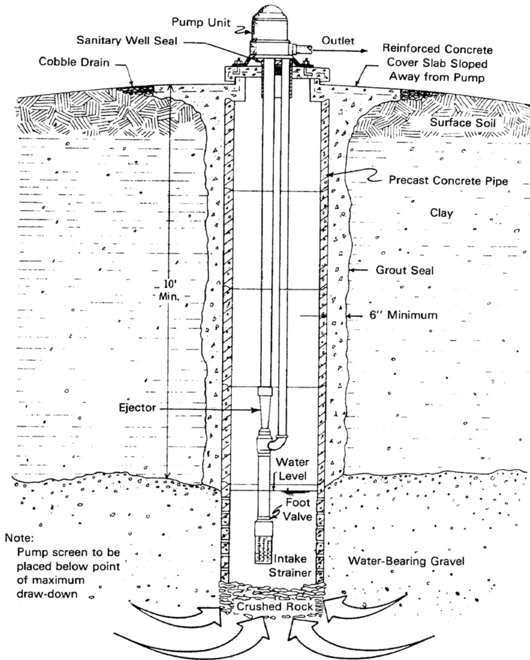
Figure 15. Dug Well with Two-Pipe Jet Pump Installation
