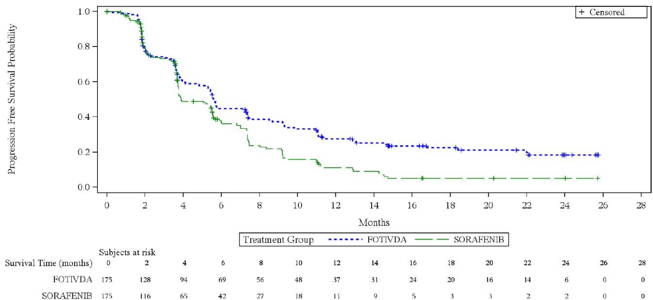
Figure 1. Kaplan-Meier Plot of PFS in TIVO-3
